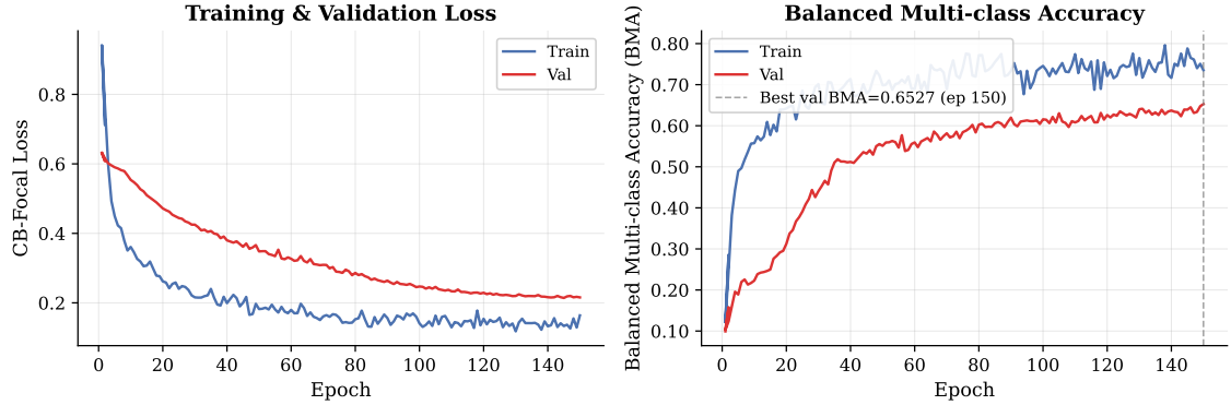
Figure 5.3: Training and validation loss (left) and BMA (right) for the DEKAN model over 150 epochs. The dashed line marks the best validation BMA.
